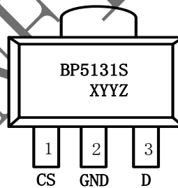
Fig 2 BP5131S Pin Mapping
